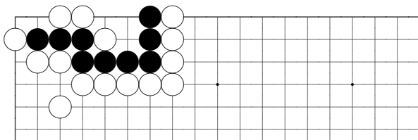
problem 755
