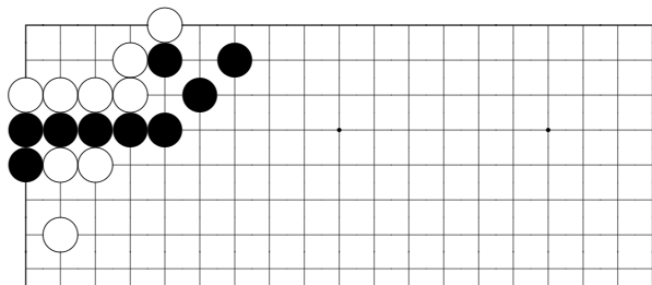
problem 372
