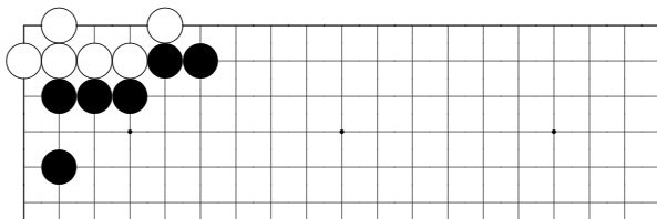
problem 6
