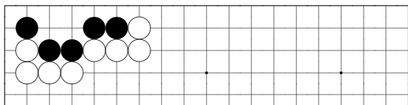
problem 235
