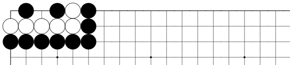
problem 5
