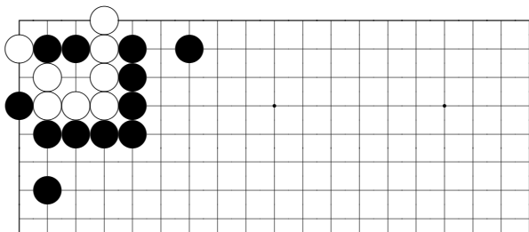
problem 647
