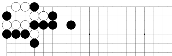
problem 161
