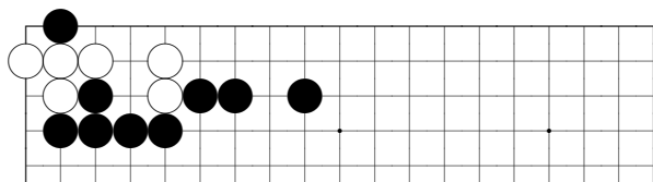
problem 310
