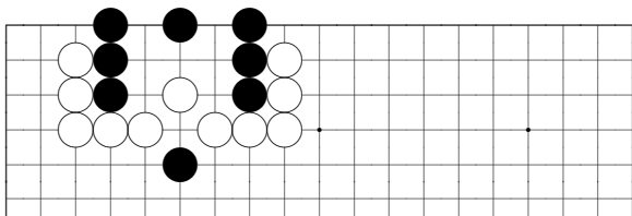
problem 864
