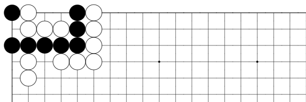
problem 548
