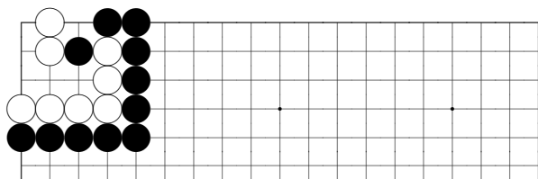
problem 615
