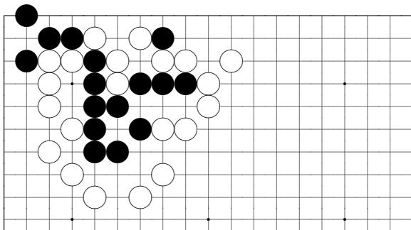
problem 898
