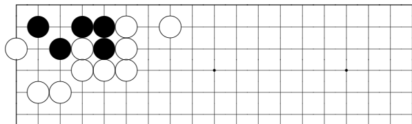
problem 225
