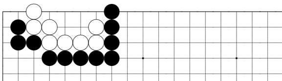
problem 757
