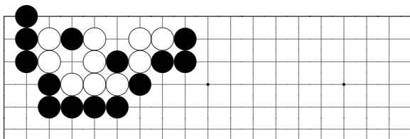
problem 855
