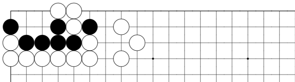
problem 379
