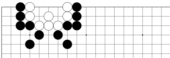
problem 708
