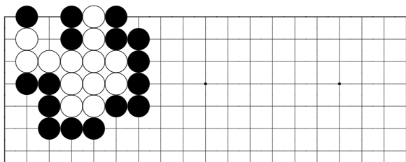
problem 298
