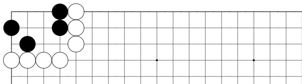
problem 95
