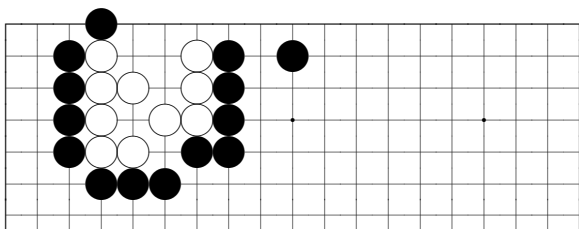
problem 836
