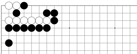
problem 583
