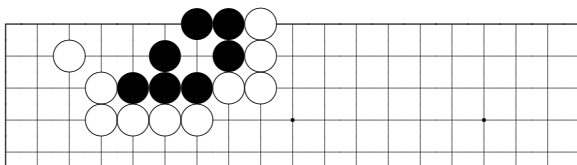
problem 707
