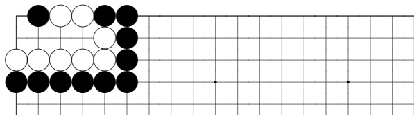
problem 532
