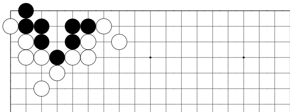
problem 46
