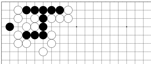
problem 77
