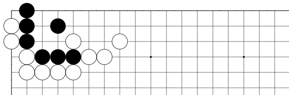
problem 773
