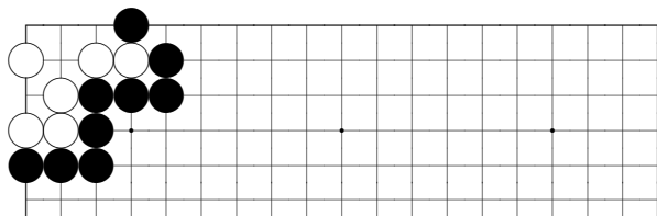
problem 110
