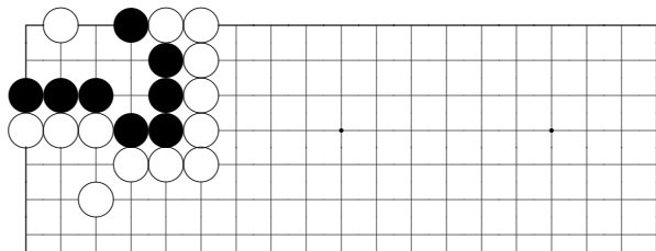
problem 424
