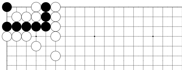
problem 545
