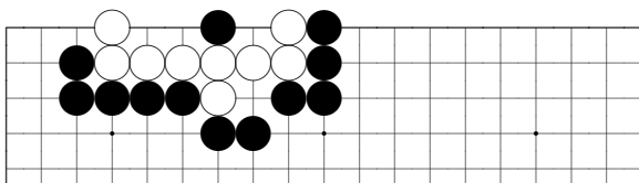
problem 669
