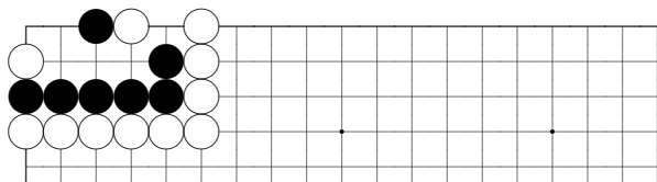
problem 539
