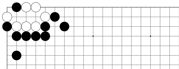
problem 447
