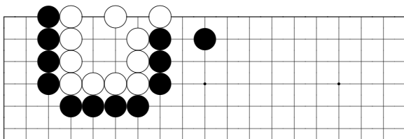
problem 803
