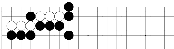
problem 493
