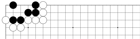
problem 159
