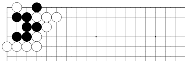
problem 361
