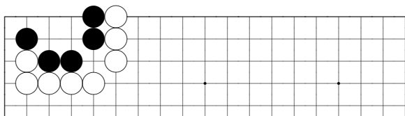
problem 236
