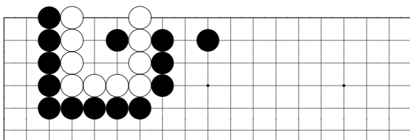
problem 790
