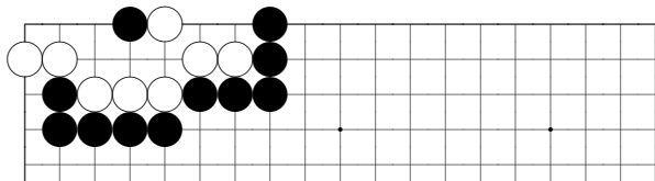
problem 292
