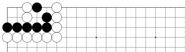
problem 499
