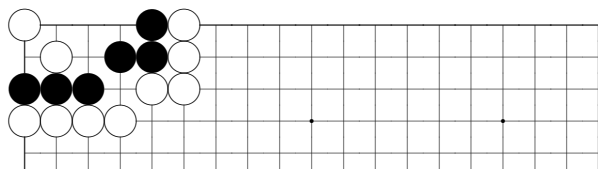
problem 194
