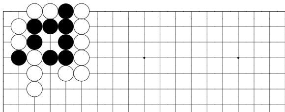
problem 104
