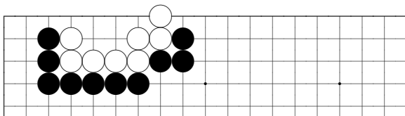
problem 673
