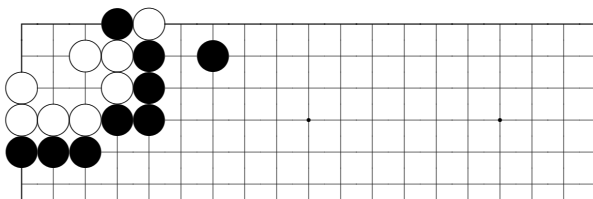
problem 605
