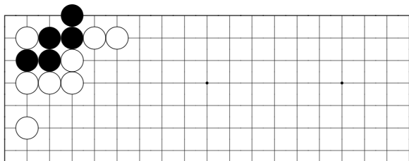
problem 154
