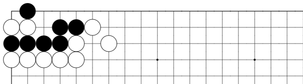
problem 507
