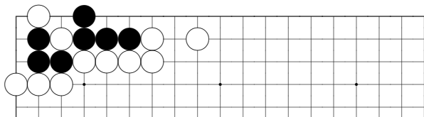
problem 145
