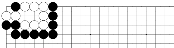
problem 246
