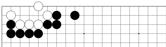
problem 553
