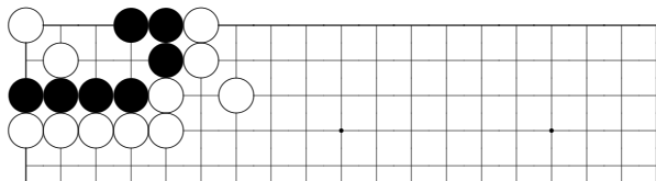
problem 468
