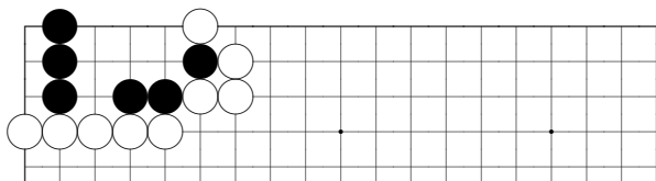
problem 51
