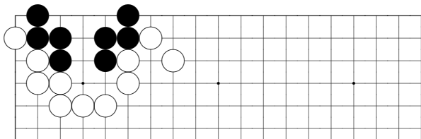
problem 84
