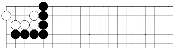
problem 366
