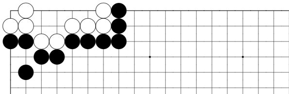
problem 303
