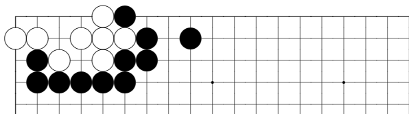
problem 89
