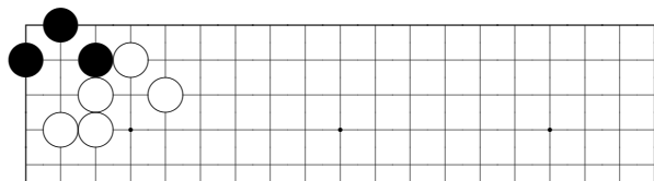
problem 117
