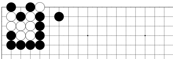
problem 652
