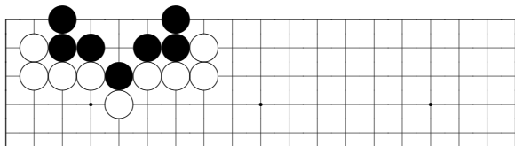
problem 81
