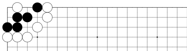
problem 112
