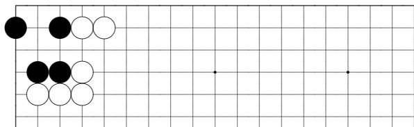
problem 325
