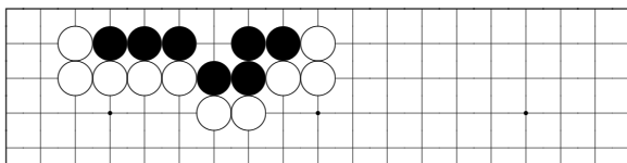
problem 672
