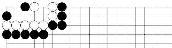
problem 587
