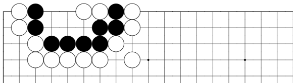
problem 723
