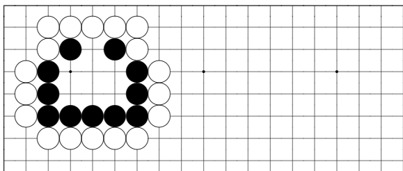
problem 889
