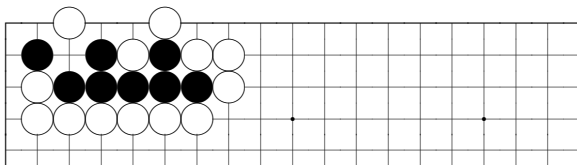
problem 709
