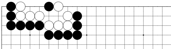
problem 692
