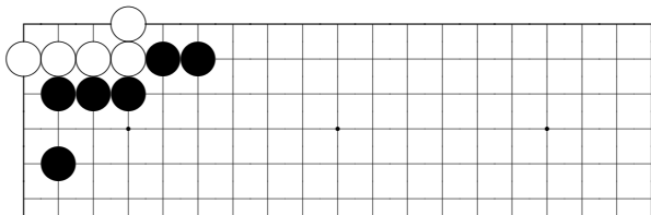
problem 1
